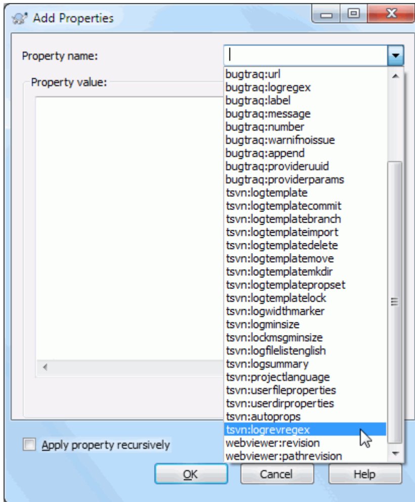
Figure 4.35. Adding properties
