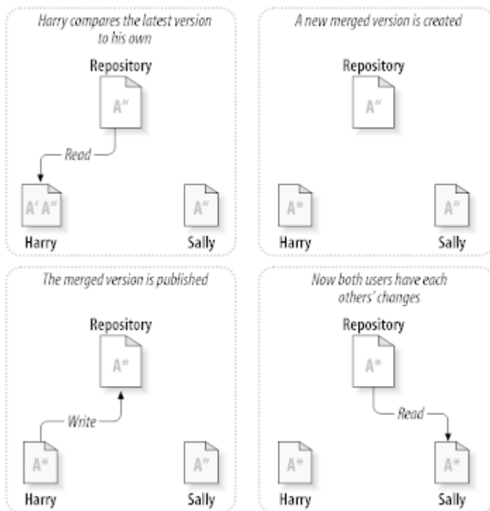
Figure 2.5. ...Copy-Modify-Merge Continued
