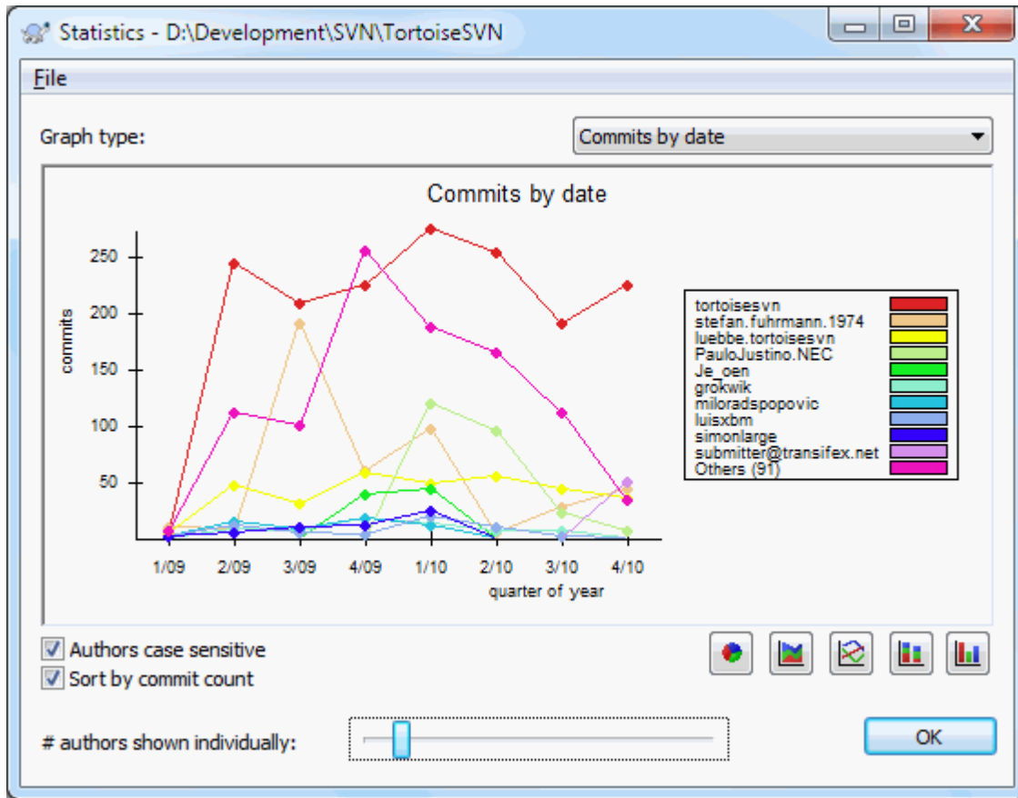
Figure 4.25. Commits-by-date Graph
