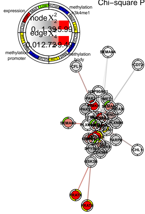
Chi-square P-value= 0.004
