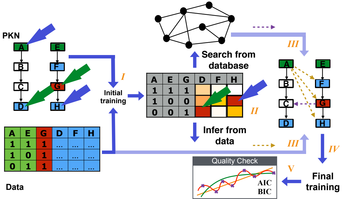
Figure 4: Dynamic-Feeder pipeline.
