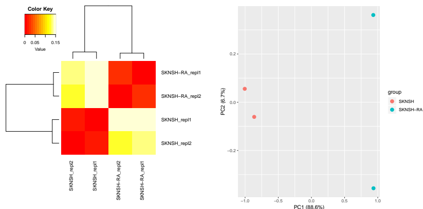
Figure 6: Quality control plots on alternative data
