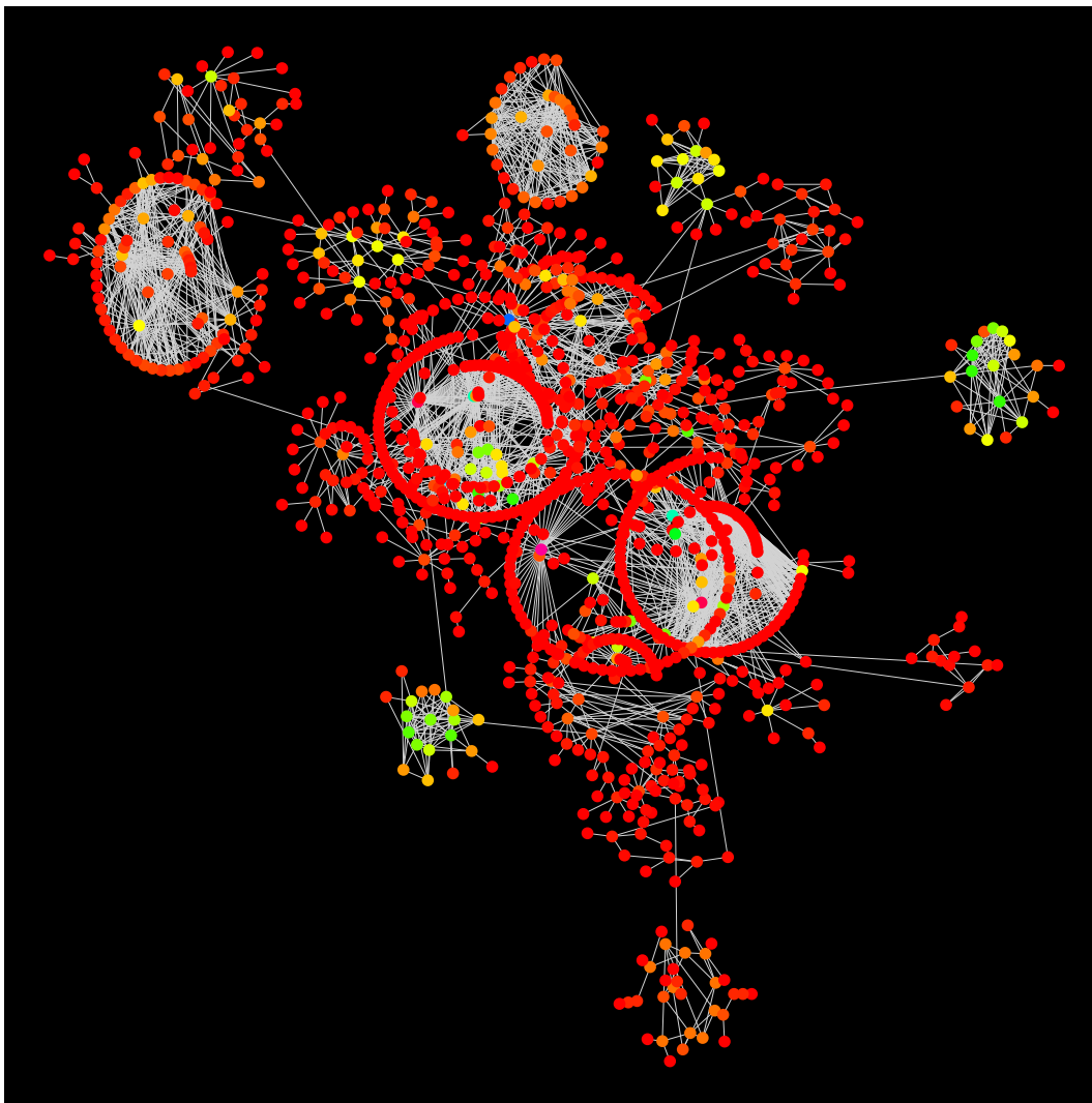
Figure 19: Modular layout of the A. Thaliana network. The position of the nodes for each module is determined by a circular tree view. Nodes in each modules are colored based on their degree according to a range of colors provided as an input. For example, nodes in module 2 are colored by a range of heat-colors, where dark colors indicate a high degree and light colors are indicating a low degree.
