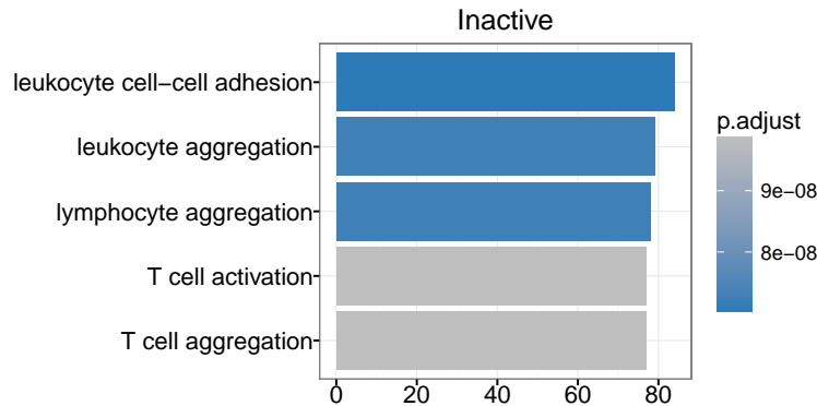
Figure 3: Example of top 5 significantly enriched Gene Ontology terms in the Inactive category. The shade of colors represents enrichment p-values and bar length represents the count of genes involved in each GO term.
