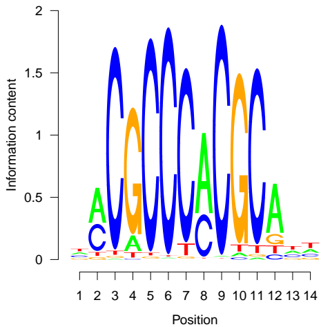
(a) Mmusculus-UniPROBE-Zif268.UP00400
