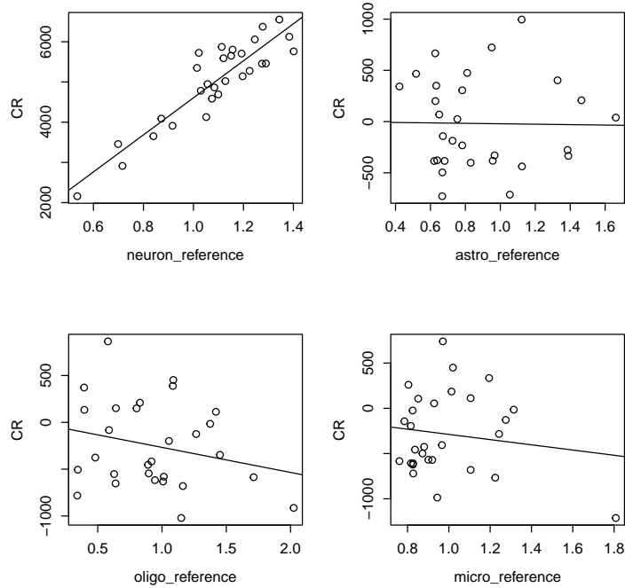
Figure 1: Component-plus-residual plots showing deconvolved neuronal, astrocytic, oligodendrocytic and microglial expression of Calceurin A in control samples.
