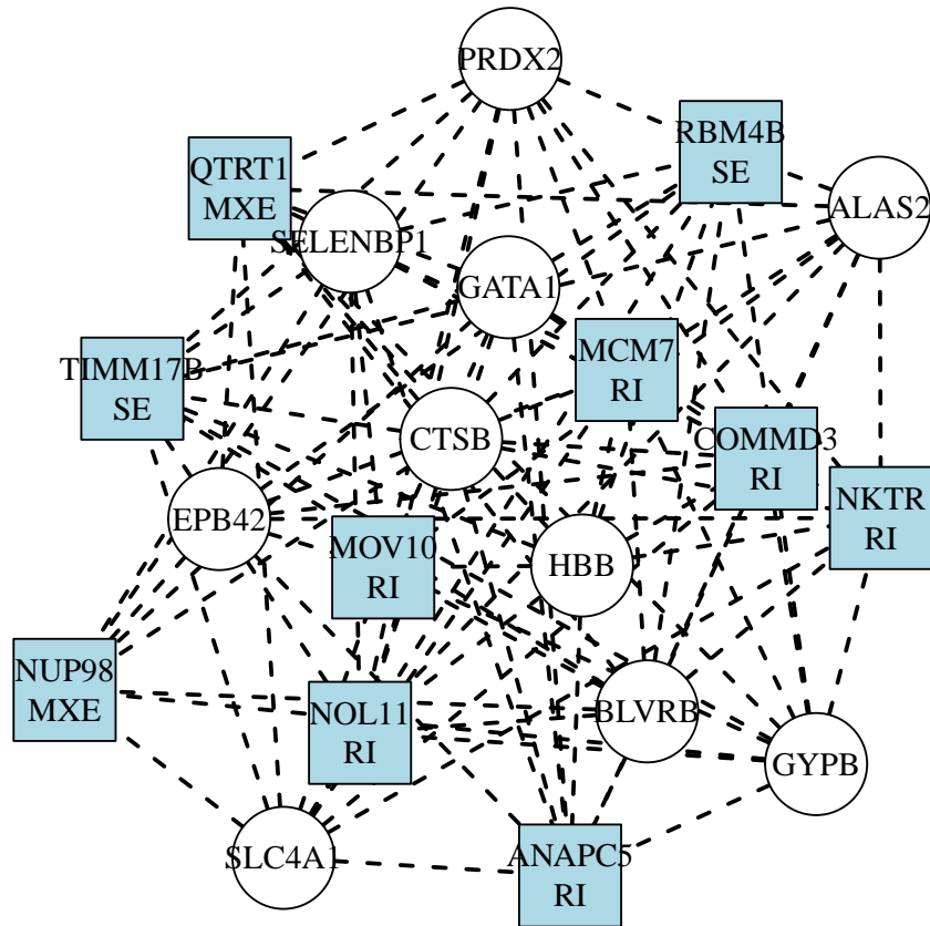
Figure 4: Pathway visualization
