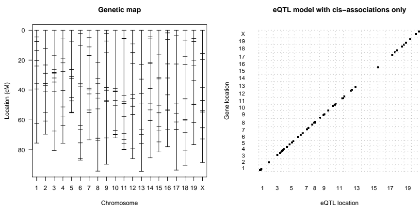
Figure 4: A genetic map simulated with the qtl package (Broman et al., 2003) on the left, and on the right, an eQTL model simulated using the genetic map with the qgraph package
