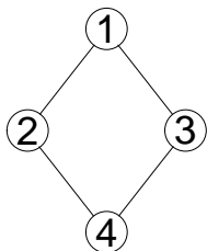
Figure 2: A 4-cycle undirected graph
