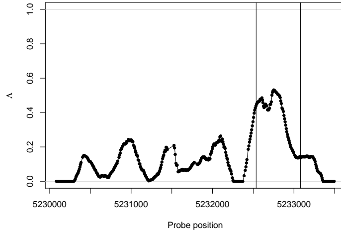
Figure 2: Results with triangular window.
