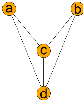
Figure 1: The graph g1 .
