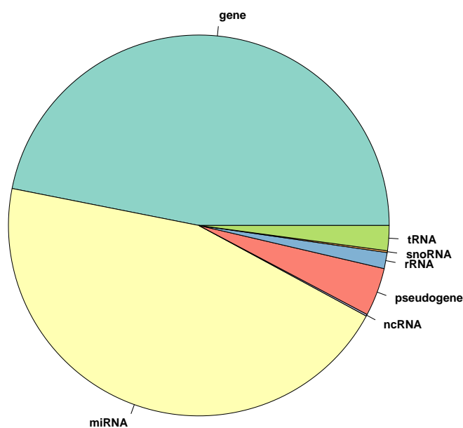
Figure 2: Pie chart showing what kinds of genome elements are overlapped by aligned reads. Note that the proportions of the pie chart are given by the proportions among all annotated genome elements that have geq1 reads mapped to them and not by the total numbers of reads mapped to elements of that class, in which case the proportion of the miRNA class would be significantly larger.
