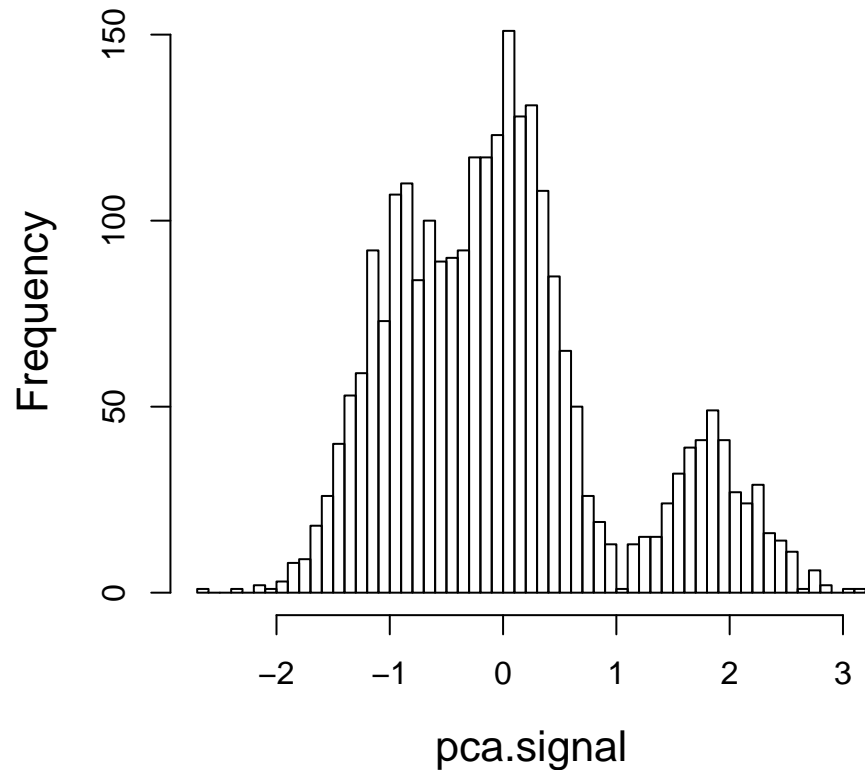
First PCA signal
