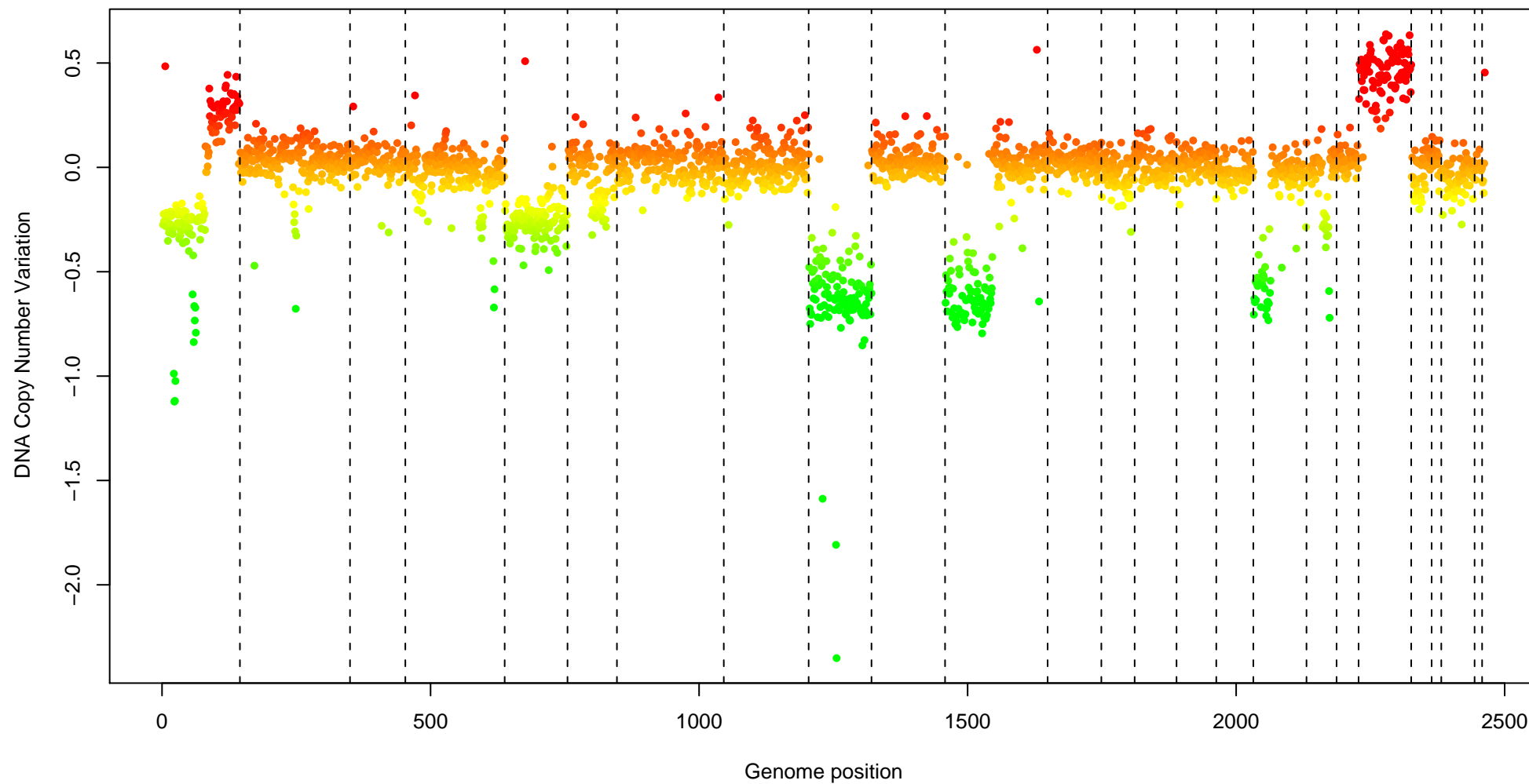
Pan-genomic representation
