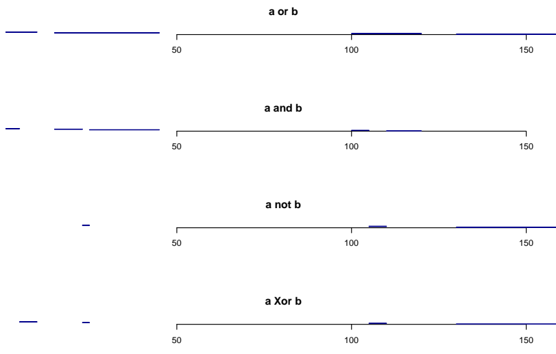
Figure 3: Union, intersection, subtraction on segments set.
