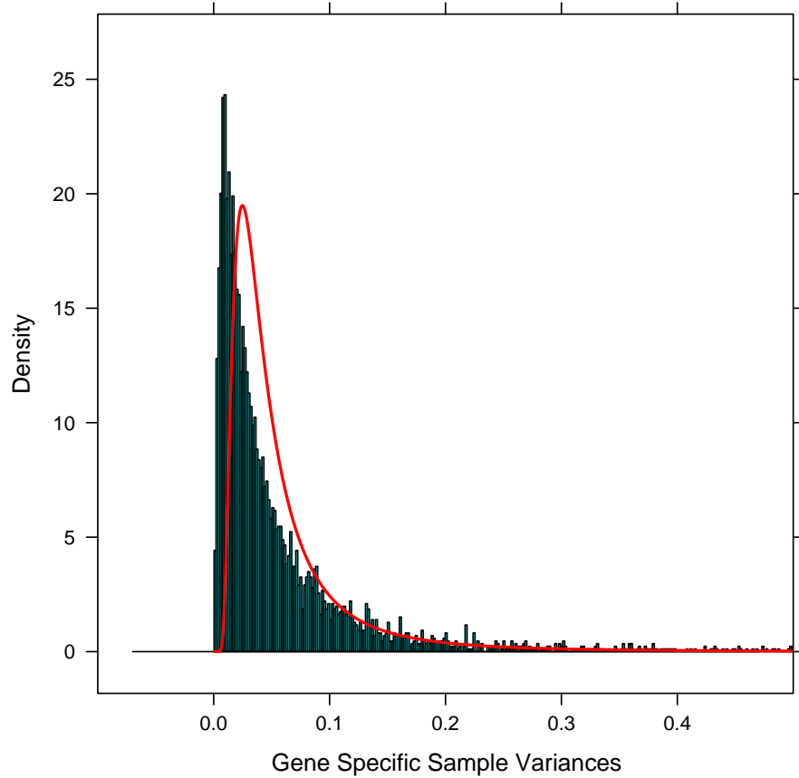
Figure 11: Density histogram of gene specific sample variances and the scaled inverse chi-square density plot (red line).
