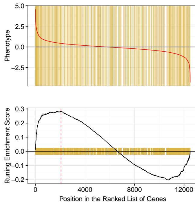
Figure 5: gseaplot example.
