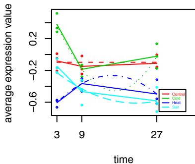
Cluster 1
