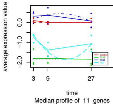
Cluster 5
