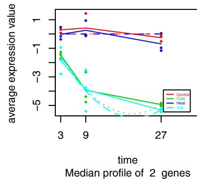
Cluster 6
