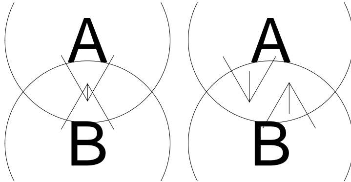
Figure 3: rEG laid out with recipEdges set to combined (left) and distinct (right).
