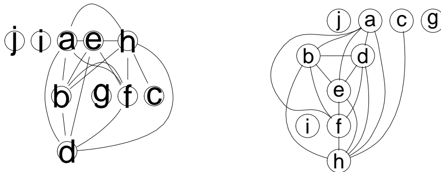
Figure 4: g1 laid out with two different settings for the parameter subGList .
