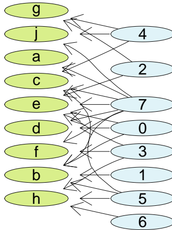
Figure 14: A bipartite graph.
