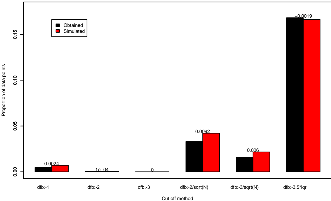
Proportion of outliers in regression assessment using dfbetas
