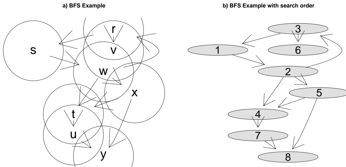
Figure 6: a) The graph for breadth-first-search example. b) The graph for breadth-first-search example, showing search orders.
