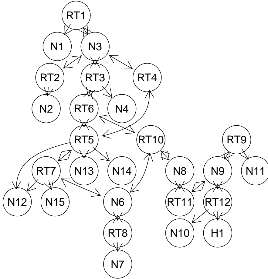
Figure 7: Network example from BGL.
