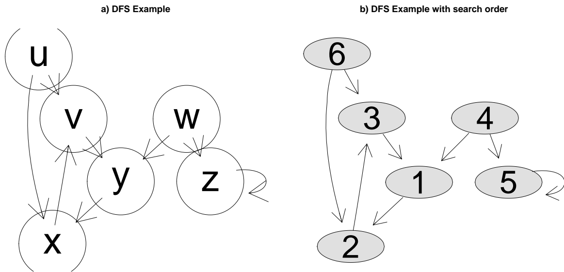
Figure 5: a) The graph for depth-first-search example. b) The graph for depth-first-search example, showing search orders.
