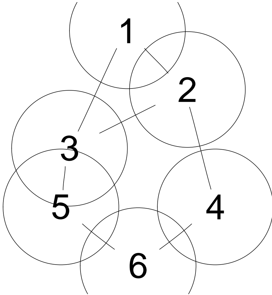
Figure 15: K-cliques Example.
