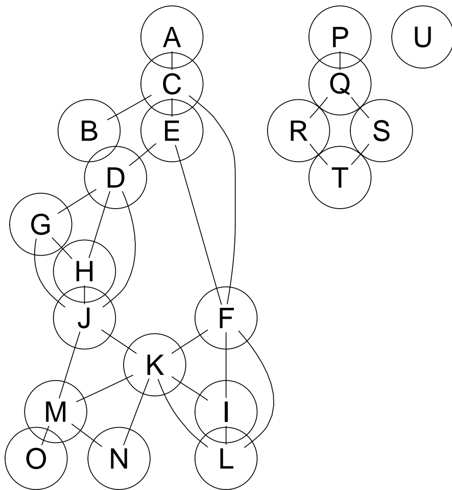
Figure 14: K-cores Example.
