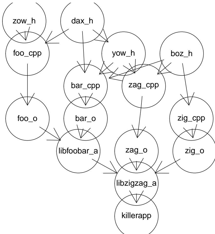
Figure 4: File dependency digraph example from Boost library.
