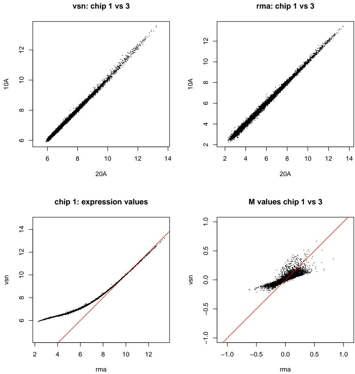
Figure 6: Results of justvsn and rma on the Dilution example data. Chip 1 was hybridised with 20 \mu\text{g} RNA from liver, Chip 3 with 10 \mu\text{g} of the same RNA.
