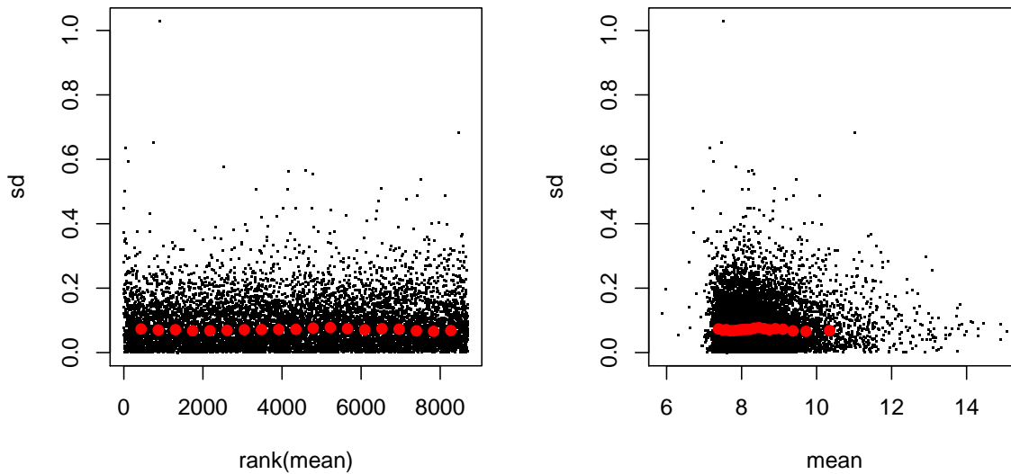
Figure 2: Standard deviation versus rank of the mean, and the mean, respectively.
