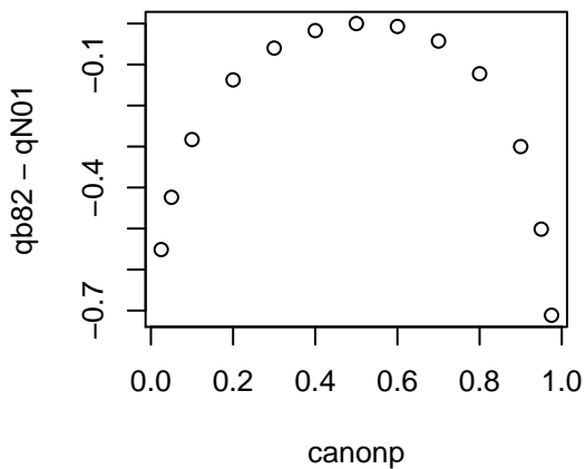
Beta(8,2)
