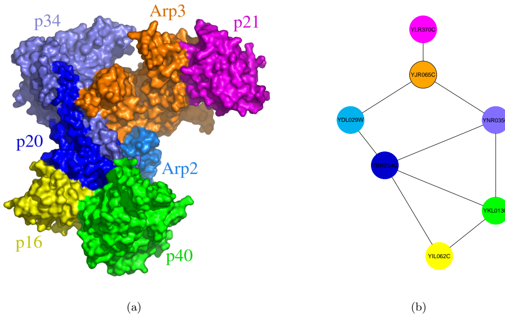
Figure 2: Some scientists might find the physical rendering of ARP 2/3 to be of more use while others might prefer a graphical representation. We note that the issue of identifiability presents itself as creator of the atomic rendering has chosen one version of the common names while the creator of the graph has chosen the systematic gene names. The coloring scheme provided allows for one to one matching of proteins from one rendering to the other.
