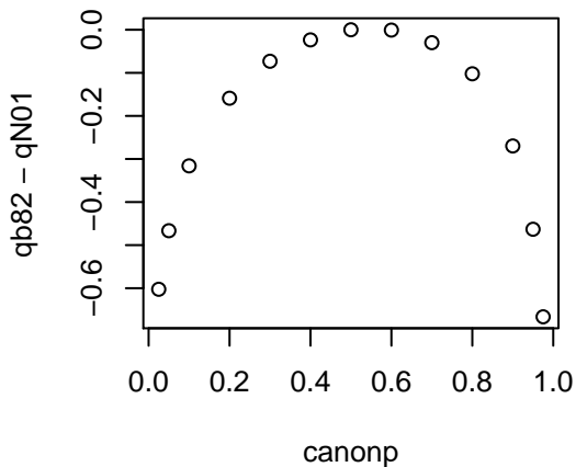
Beta(8,2)
