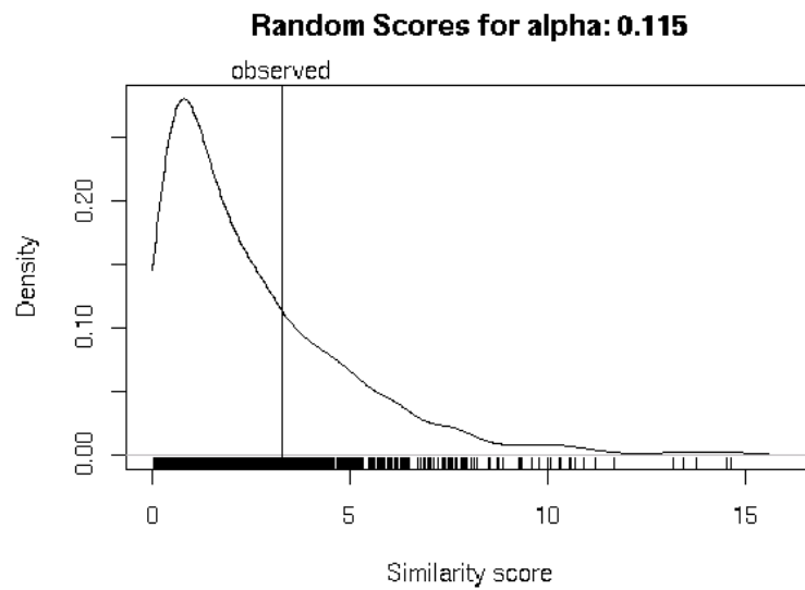
Figure 4.2: plot(z,"density") : Shown are kernel density estimates of the distribution of random similarity scores. The observed score is marked by the vertical line.
