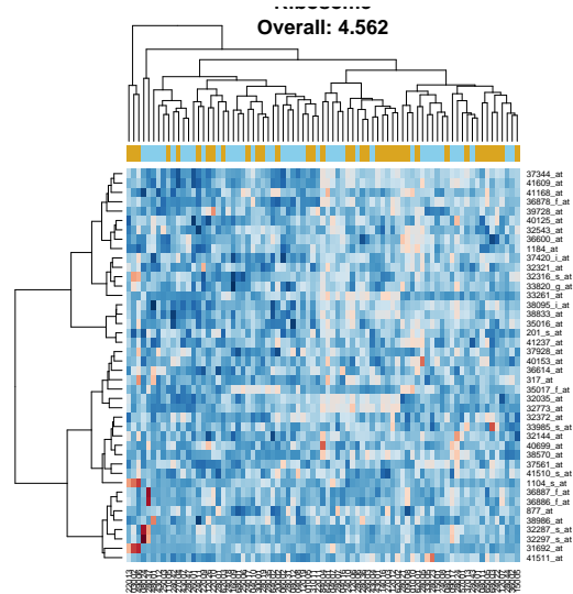
Figure 4: The mean plot for the category with the smallest p-value.
