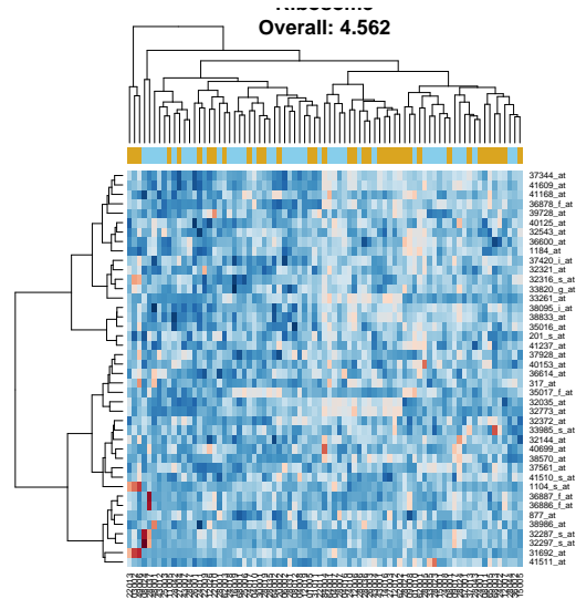
Figure 2: The mean plot for the category with the smallest p-value.
