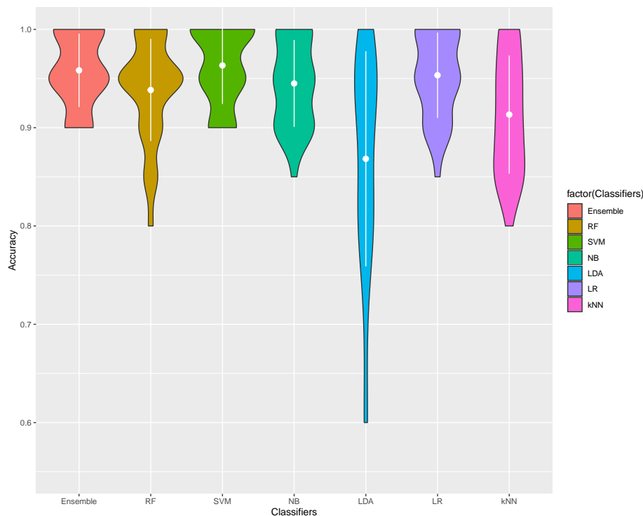
Figure 18: Accuracies Comparison
