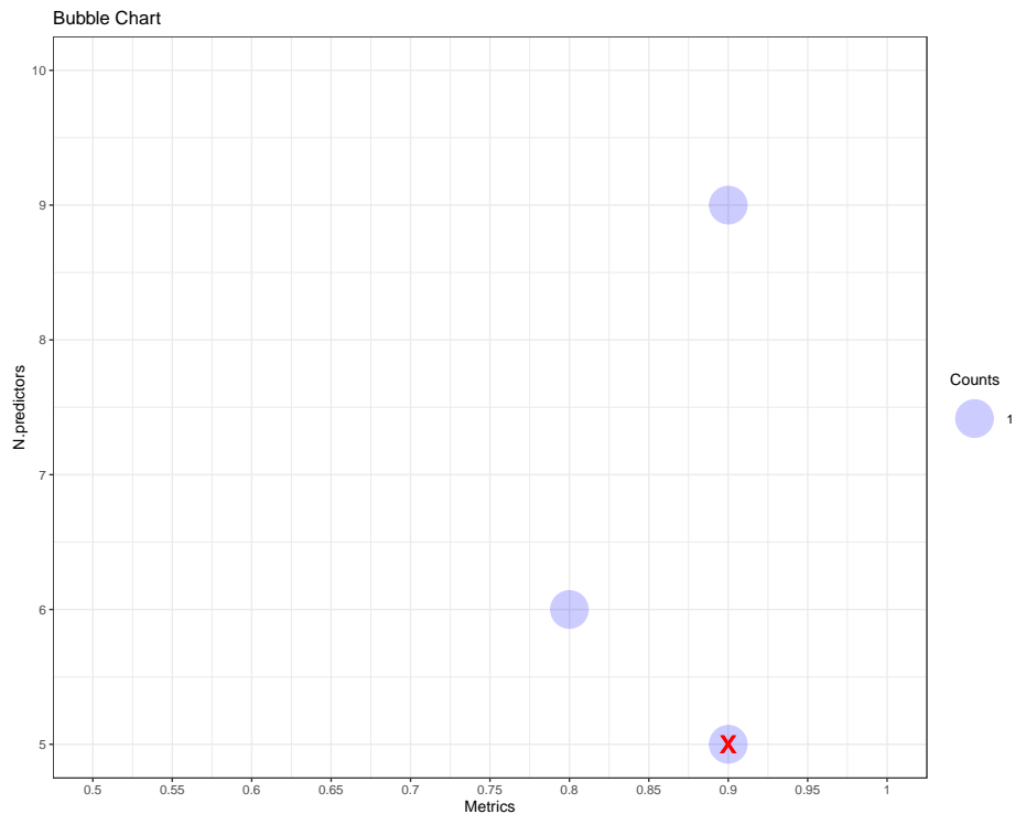
Figure 15: Bubble Chart
