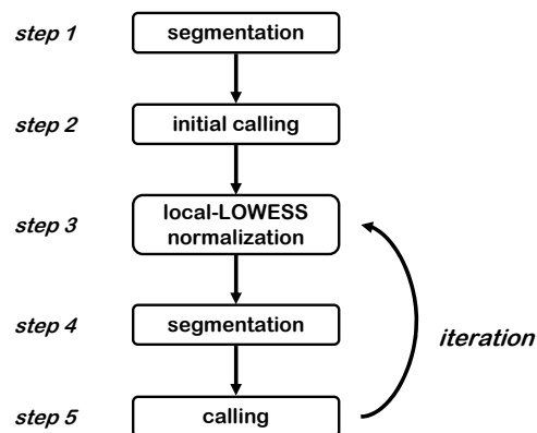
Figure 1: Overview of the CGHnormaliter method.
